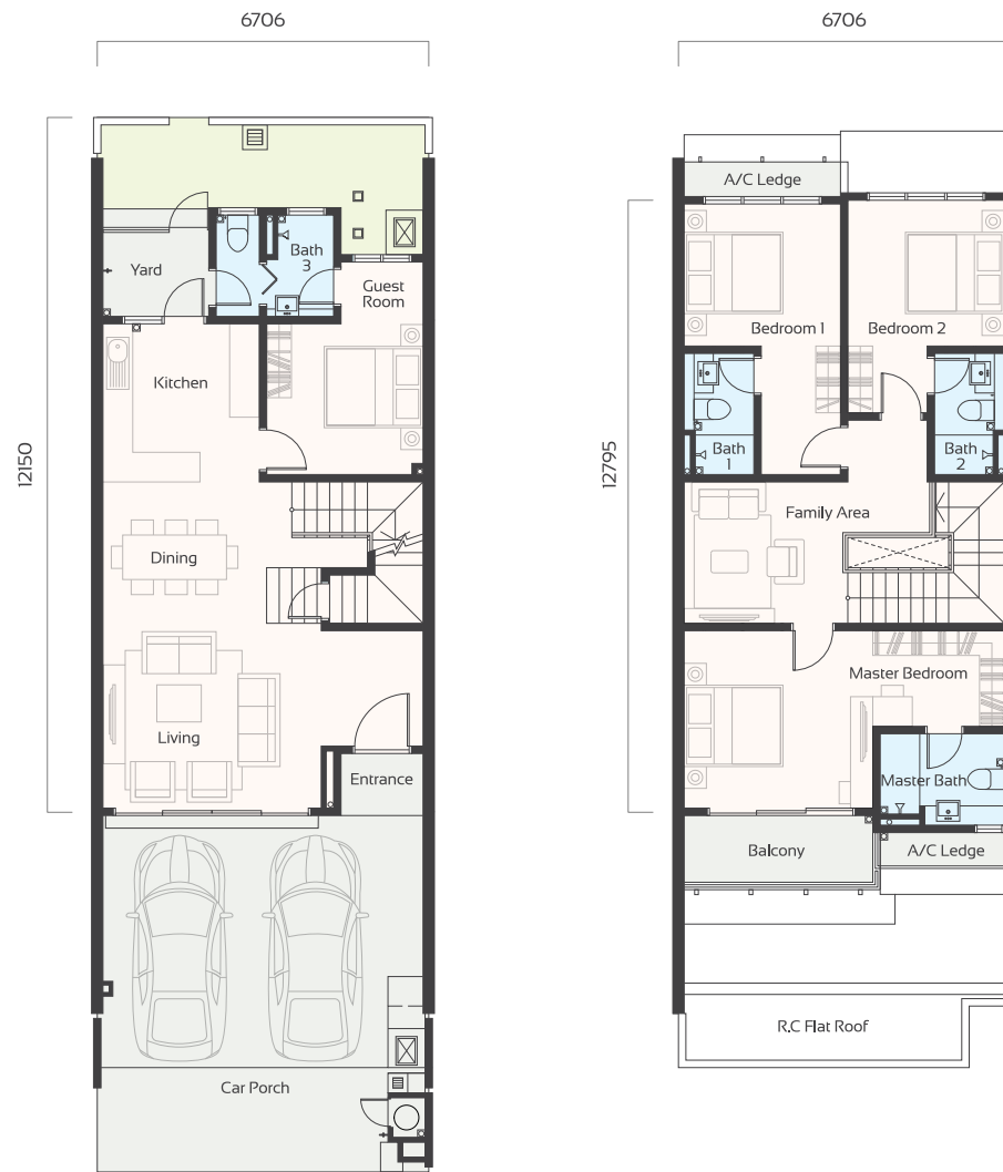
GROUND FLOOR
